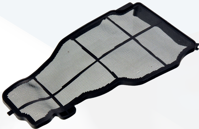
ADBP250047 Cabin Filter (for high voltage battery compartment) OE No. G92DH-47060 To fit: Toyota Prius (2008-2016)
